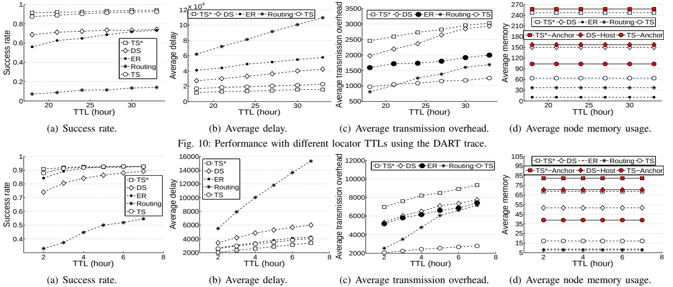
Fig. 11: Performance with different locator TTLs using the DNET trace.
